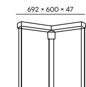
Canopy for PC1133 incl. PWM dimming system
