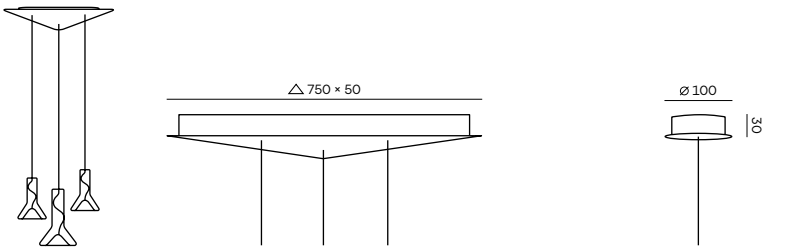
PC961 Canopy for PC961 Canopy for single lights
