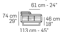
Laterale/Depth
