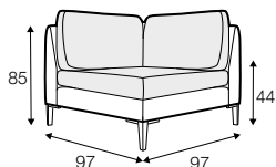
corner 90° no. 1
