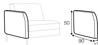
armrest C
